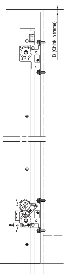
Position diagram for Close assist device and rail mounting holes (as viewed from inspection panel) M5 (P=0.8)
