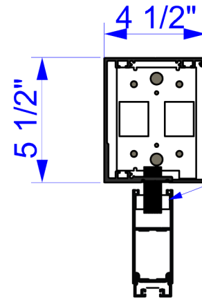
VERTICAL SECTION
